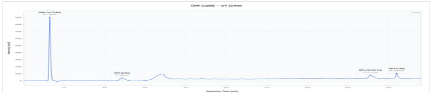
KLOW 80mg - RNV-KLOW-2607A: UV Chromatogram
