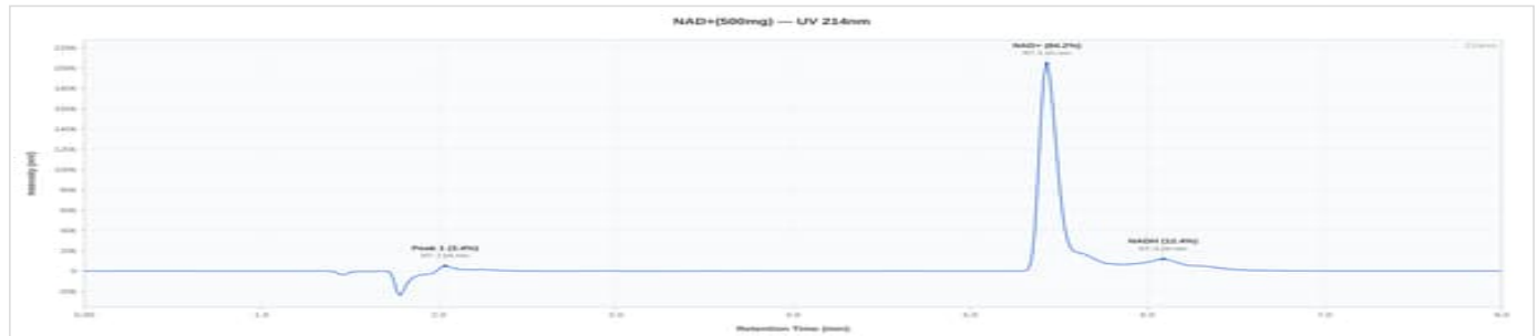
NAD+ 500mg - RNV-NAD-2603A: UV Chromatogram
