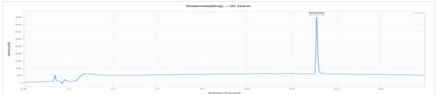
Retatrutide 40mg - RNV-RETA-2808A: UV Chromatogram
