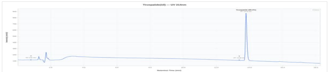
Tirzepatide 10mg - RNV-TIRZ-2607A: UV Chromatogram
